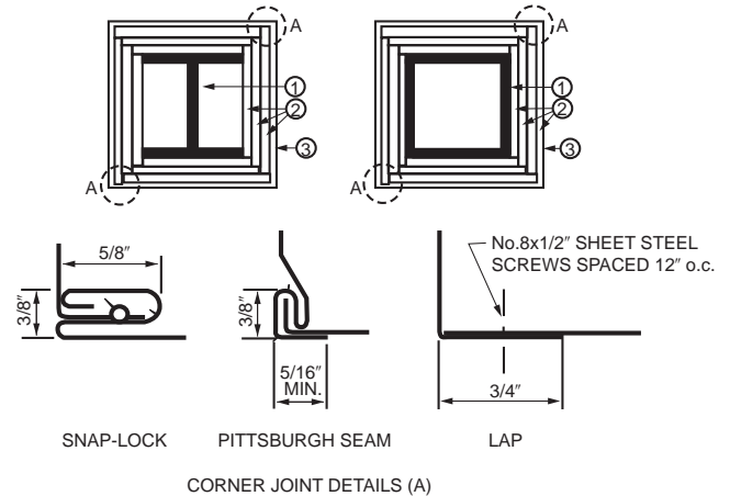
FIGURE 722.5.1(2) GYPSUM-PROTECTED STRUCTURAL STEEL COLUMNS WITH SHEET STEEL COLUMN COVERS
