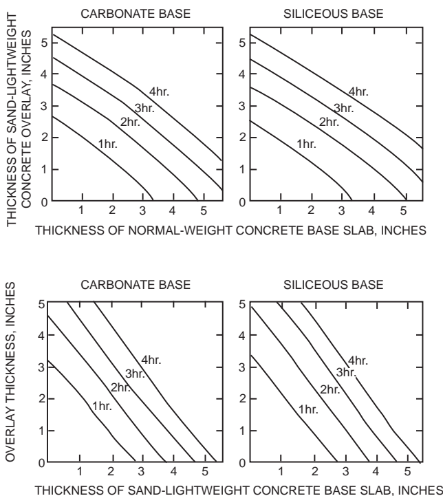
FIGURE 722.2.2 FIRE-RESISTANCE RATINGS FOR TWO-COURSE CONCRETE FLOORS
